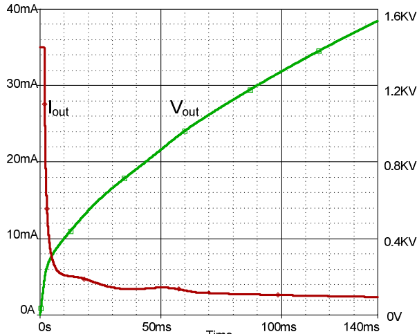
Fig. 14. Simulation results of one charging cycle obtained by the circuit of Fig. 13 – Capacitor charging current and voltage versus time.
