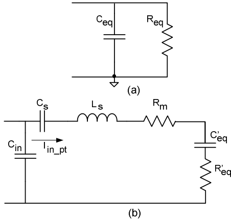
Fig. 9. (a) Equivalent RC circuit of the voltage doubler of Fig. 2 at a given frequency \omega . (b) Series equivalent circuit of a PT connected to a voltage doubler.
