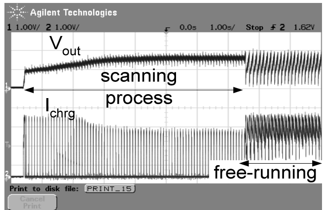
Fig. 5. Experimental results showing the concept of proposed capacitor charger control. Upper trace: output voltage 750V/div. Lower trace: Charging current 3mA/div. Horizontal scale 1s/div.
