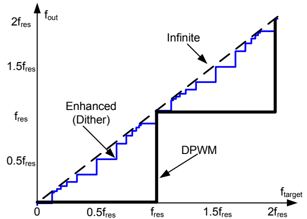
Fig. 7. Output frequency versus desired frequency for original DPWM and 3 bit resolution enhancement.
