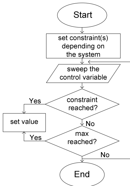
Fig. 1 Conceptual flow chart of proposed search-and-tune algorithm for generating the optimal charging profile.
