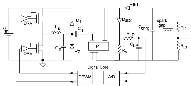
Fig. 6. Experimental setup.
