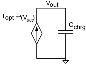
Fig. 13. Behavioral current-source model used to simulate the optimal charging process of the output capacitor.
