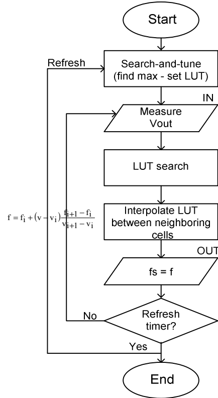
Fig. 4. Detailed flow chart of the main routine of proposed control method.
