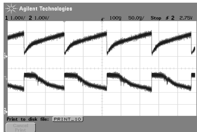
Fig. 16. Experimental results of free running operation with 3bits frequency resolution enhancement on the basic 1kHz resolution. Upper trace: output voltage (750V/div). Lower trace: Charging current (3mA/div). Horizontal scale 50ms/div.
