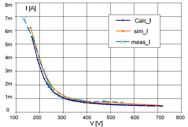
Fig. 12. Calculated, simulated and measured maximum charging current as a function of the output voltage.
