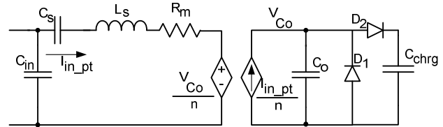
Fig. 2. Equivalent circuit of piezoelectric transformer (PT) connected to a voltage doubler rectifier.
