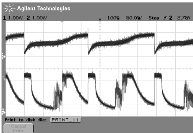
Fig. 15. Experimental results of free running operation with a frequency resolution of 1kHz. Upper trace: output voltage (750V/div). Lower trace: Charging current (3mA/div). Horizontal scale 50ms/div.
