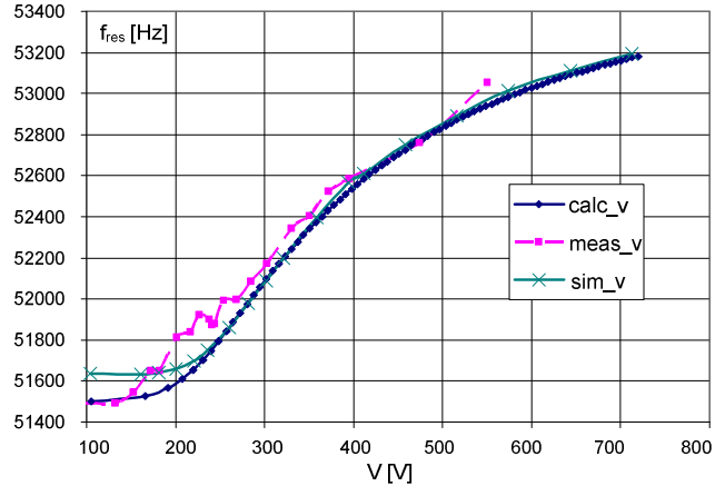
Fig. 11. Calculated, simulated and measured resonant frequency variation as a function of the output voltage.
