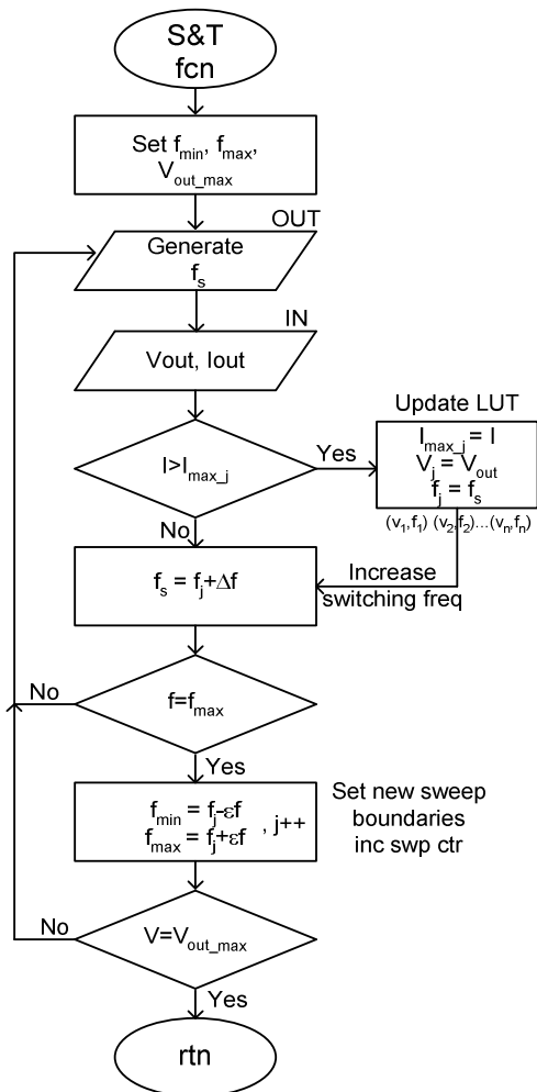
Fig. 3. Detailed flow chart of the search-and-tune routine for generating the optimal charging profile.
