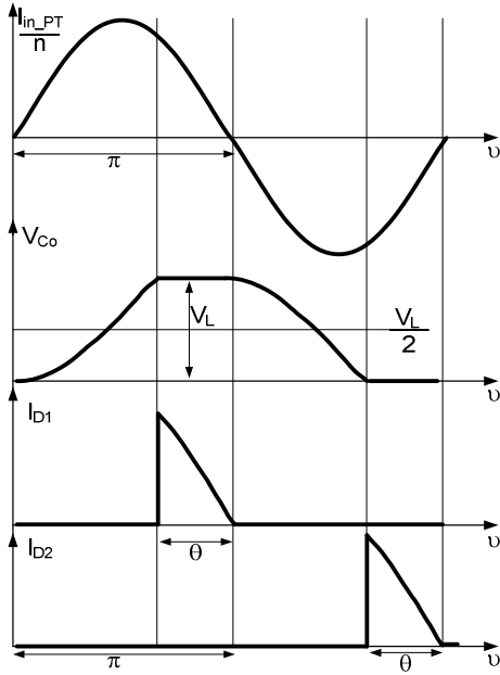
Fig. 8. Typical current and voltage waveforms of the voltage doubler rectifier fed by a piezoelectric transformer (Fig. 2).
